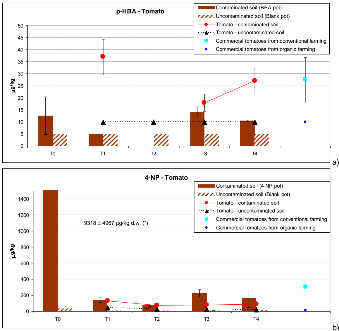
Figure 2: p-HBA (a) and 4-NP (b) concentrations in soil ( \mu\text{g}/\text{kg} d.w.) and tomatoes ( \mu\text{g}/\text{kg} f.w.) from the tomato pots, and in the commercial samples.
